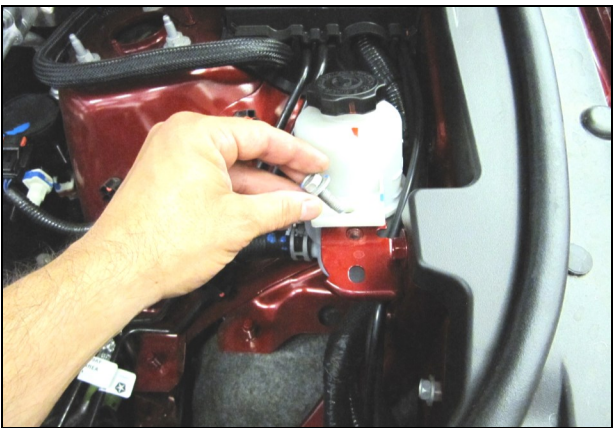
12. Remove the bolt securing the power steering reservoir and set it aside. This bolt will be reused in step 13. to hold the Mounting bracket.
