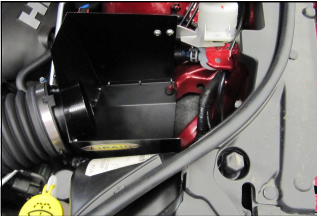
13. Install the Panel assembly into the engine compartment as shown. Slide the Mounting bracket underneath the power steering reservoir and the airbox mounting post through the grommet in the Panel. Secure the assembly by reusing the bolt from step 12. Connect the factory intake tube to the Airaid Intake tube and tighten the clamp.
