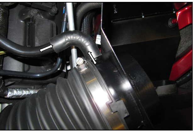
15. On V6 motors, connect the factory crankcase breather hard line to the Airaid Intake Tube using the 90 deg. Breather Elbow (#7). Disregard the 13" Breather Hose (#6) it will not be used.
