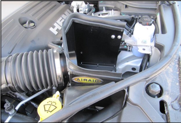
16. Install the Weather Strip (#4) to the top edge of the panels, and reattach the hood seal. Apply the Airaid Decal to the Panel Assembly.
