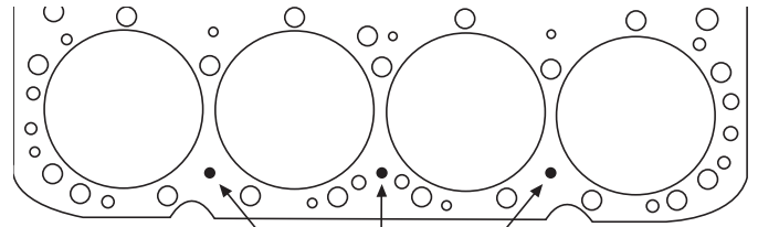
Figure 1 - Steam Hole Locations (400 C.I.D. Engines ONLY)
