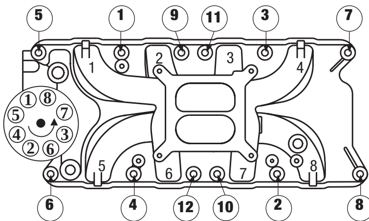
Figure 2 - 260-289-302 Ford Torque Sequence
