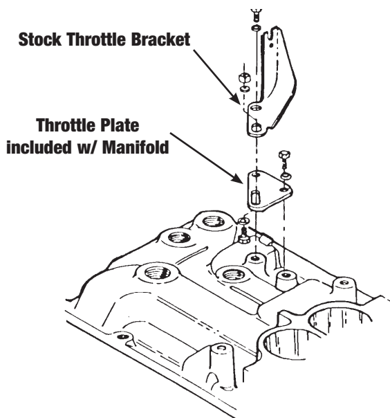
Figure 1 - Throttle Plate
