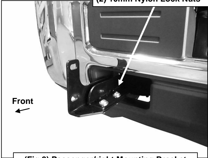
(Fig 8) Passenger/right Mounting Bracket
