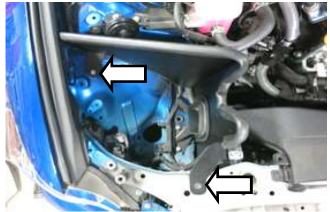
f. Place the heat shield into the engine bay, as shown above. Fasten the heat shield to the wheel well with the supplied M6 bolt and to the core support with the M6 bolt you removed in the previous step.
