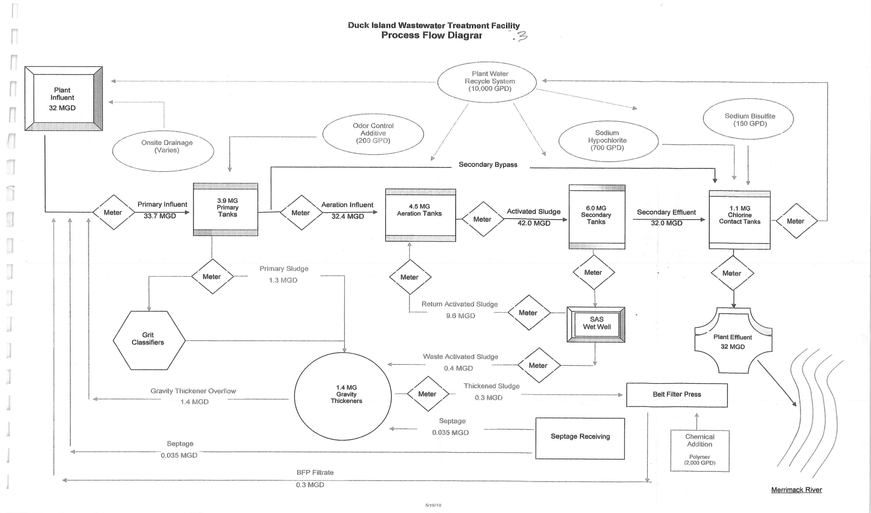
Figure 1: Flow diagram
