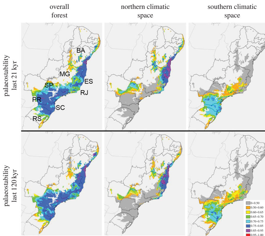
Figure 2. Forest stability models over the last 21 kyr (above) and 120 kyr (below), assuming zero forest dispersal over time (static forest refugia). Legend depicts suitability values, calculated as the sum of negative log probabilities of forest occurrence in each time period. Left panel depicts predictions when the forest is modelled as a whole. Central and right panels portray predictions for the northern and southern climatic spaces of the forest, respectively. State boundaries are included in maps; BA, Bahia; ES, Espírito Santo; MG, Minas Gerais; PR, Paraná; RJ, Rio de Janeiro; RS, Rio Grande do Sul; SC, Santa Catarina; SP, São Paulo. For models that assume forest dispersal over time, refer to the electronic supplementary material, figure S2.
