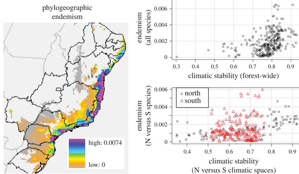
Figure 3. Phylogeographic endemism map based on available data from all AF species included in this study (left), and the relationship between phylogeographic endemism and forest stability over the last 120 kyr (right). The top graph describes how overall phylogeographic endemism relates to forest stability when the AF is modelled as a whole. The bottom graph portrays phylogeographic endemism of the northern species (black circles) and of the southern species (red triangles) in relation to forest stability values of the northern and southern climatic spaces, respectively. Stability values represent the sum of negative log probabilities of forest occurrence in each time period. Similar results are observed when values are estimated over the last 21 kyr (see the electronic supplementary material, figure S4).
