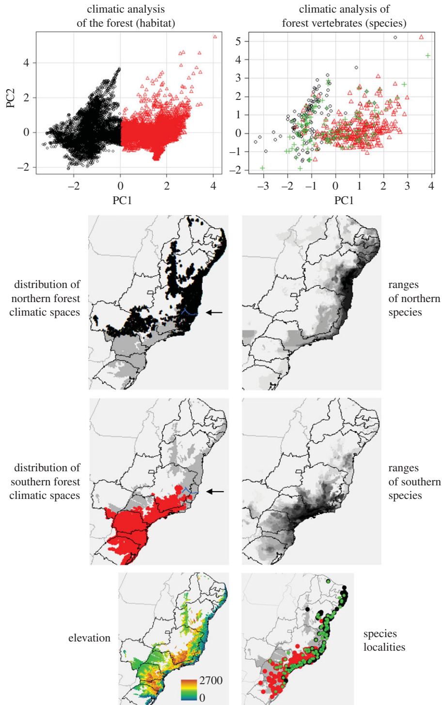
Figure 1. Left column: PCA-based identification of two climatically distinct spaces within the AF (top graph, black and red points), followed by maps of their respective northern (black) and southern (red) geographical ranges. In both maps, the areas in grey indicate the remaining extent of the forest; the location of the Rio Doce is shown with an arrow. Right column: PCA-based identification of species assemblages along the climatic axes of the AF (top), identifying the environmental spaces occupied by those taxa with northern (black), southern (red) or widespread (green) distributions. The graph is followed by maps of the superimposed ranges of the northern and southern species, respectively. In both maps, darker shades of grey represent pixels with greater species richness, as per superimposed correlative species distribution models. An elevation map is provided at the bottom of the figure (left), followed by a map of point localities of all species (right), shown over a grey mask of the AF. The colour scheme for the point localities follows that of the PCA analysis (northern species shown in black, southern taxa in red, widespread species in green).
