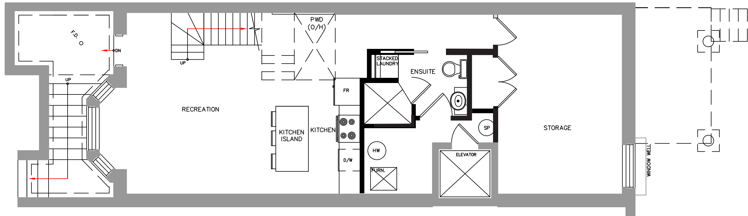
BASEMENT FLOOR CONSTRUCTION PLAN
