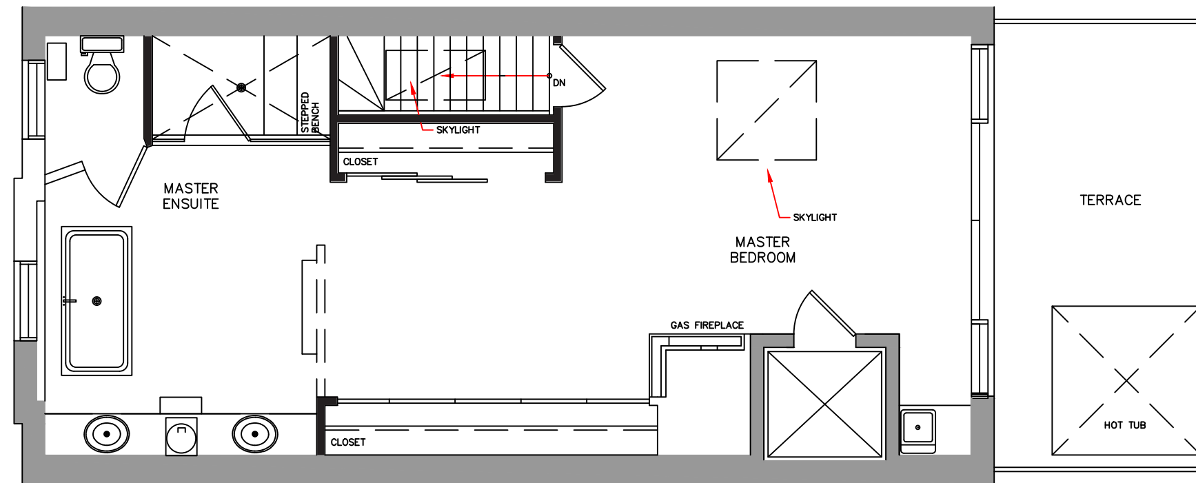
THIRD FLOOR CONSTRUCTION PLAN
