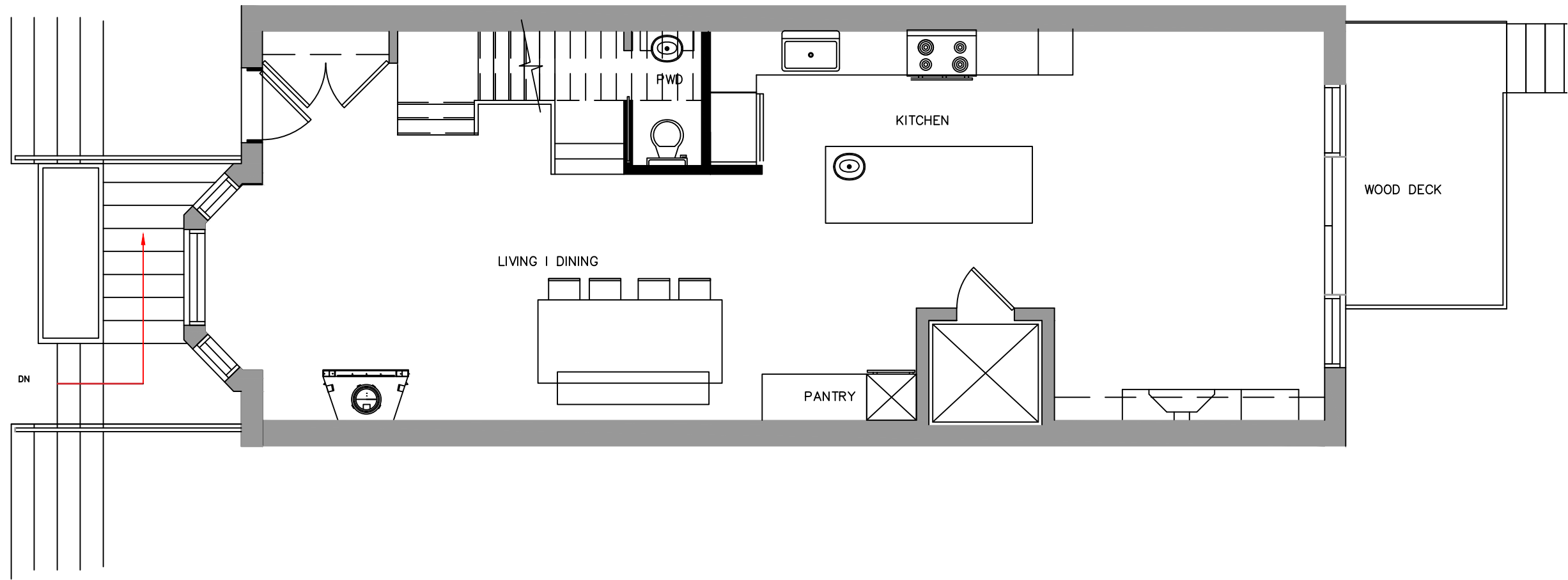
FIRST FLOOR CONSTRUCTION PLAN
