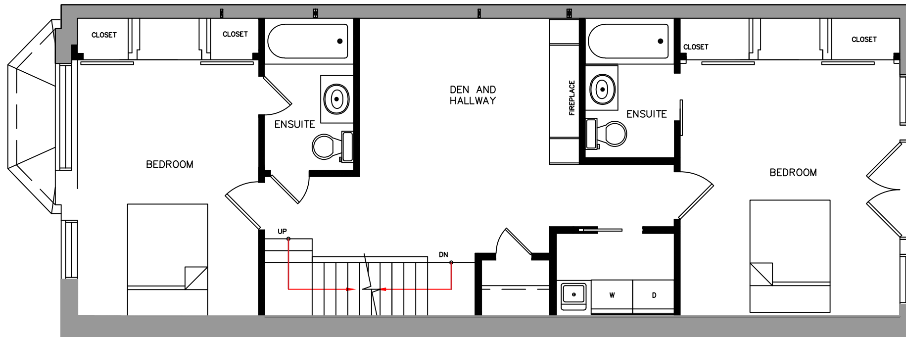
SECOND CONSTRUCTION PLAN
