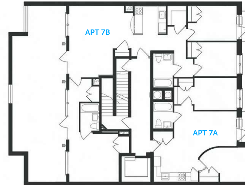
7TH FLOOR
