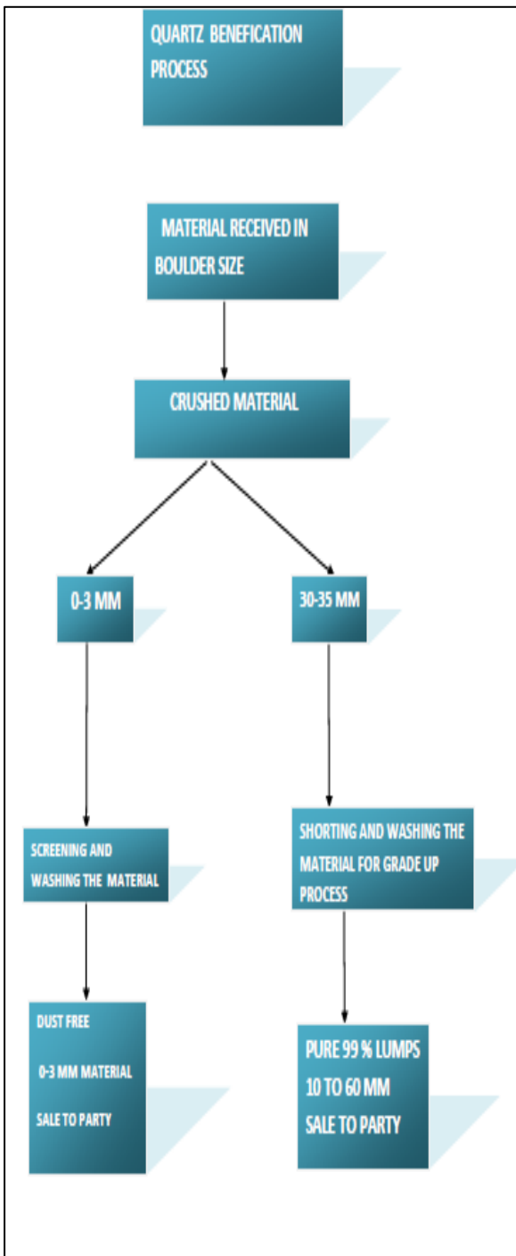
QUARTZ
