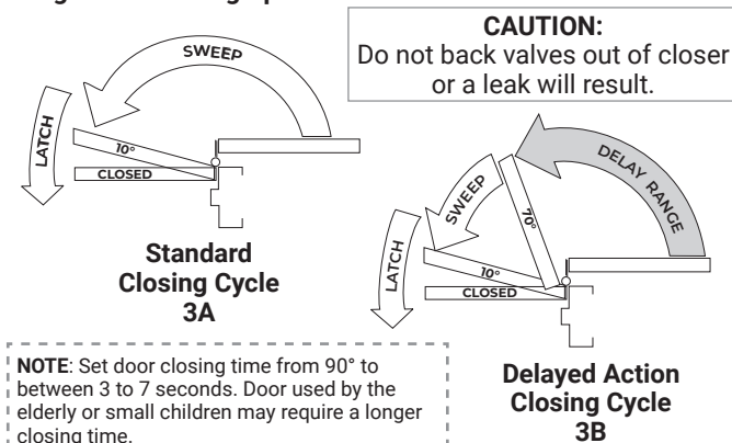
Figure 4 - Closing Speed Controls
