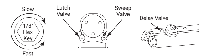
Figure 4 - Closing Speed Controls
