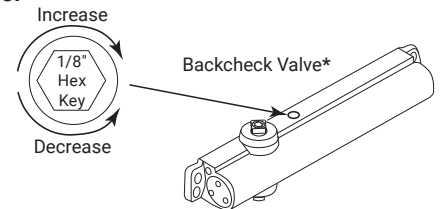
Adjustment Chart (3381 & 3581 Only)
