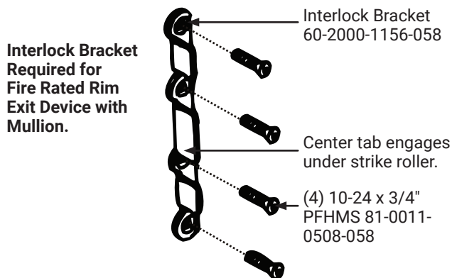
Detail F
