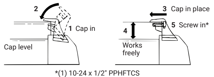
End Cap Detail
