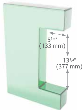
Glass Cut-Out Required for CLH-IN
