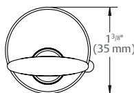
1" Thumbturn with Collar (PFD-LOCKTT)
