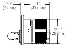
1" Thumbturn with Collar (PFD-LOCKTT)
