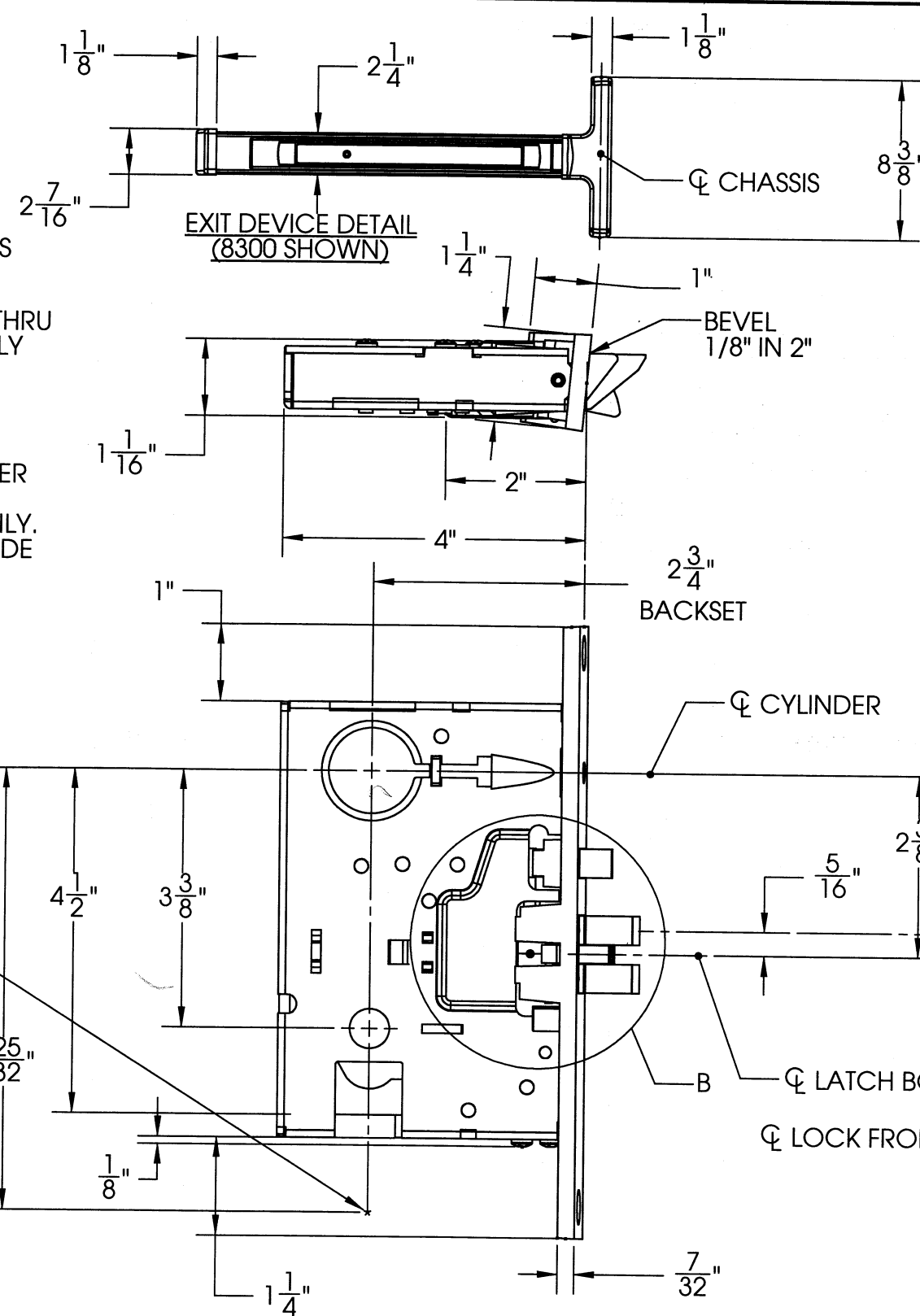
MORTISE LOCK DETAIL
