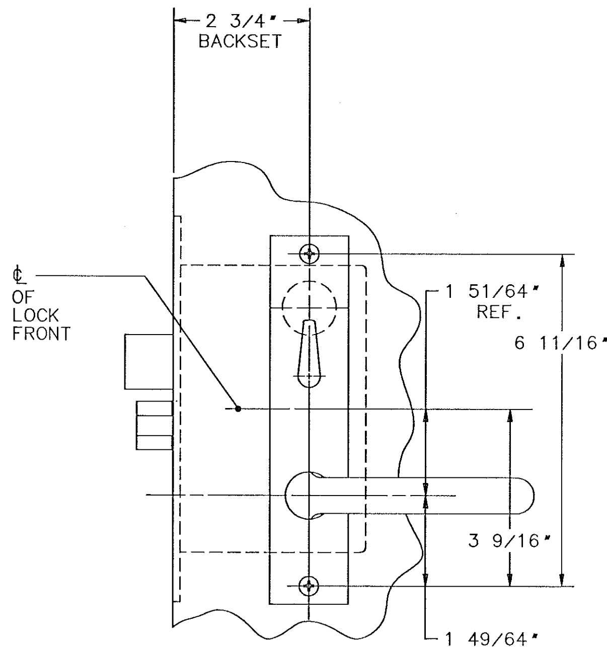
DETAIL OF INSIDE TRIM IN RELATIONSHIP TO LOCK BODY
