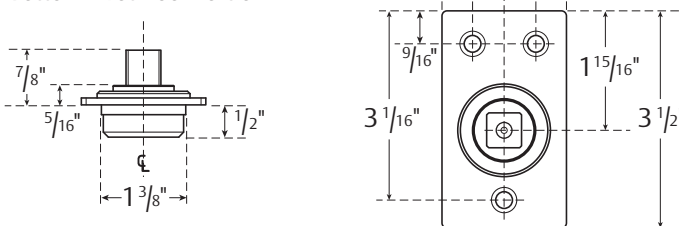
Bottom Pivot Floor Portion
