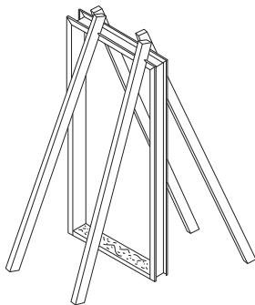
Fig. 2 – Bracing the Frame
