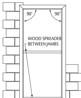
Fig. 6 – New Masonry Const.
