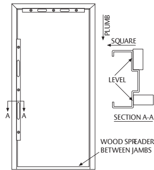
Fig. 1 – Plumbing the Frame
