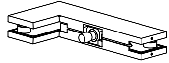
Sidelite Transom Patch (PFT-40)
