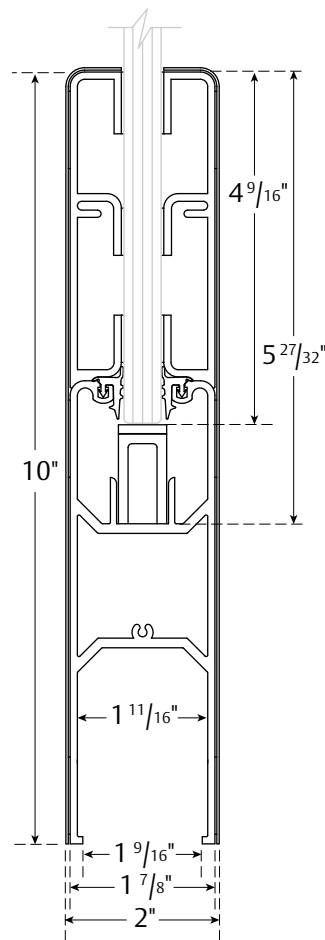
10" Sidelite Rails = 4 9/16" Bite Top and Bottom
