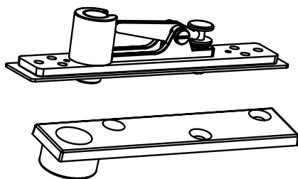
Walking Beam Pivot (PV-WALKBEAM)
