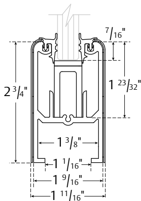
2 3/4" Square Sidelite Rails = 7/16" Bite Top and Bottom
