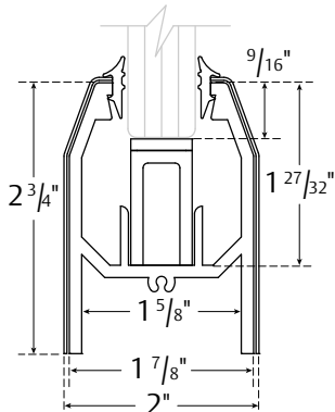
2 3/4" Tapered Sidelite Rails = 9/16" Bite Top and Bottom
