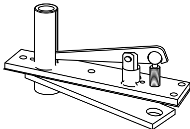
Extended Pin Walking Beam Pivot (PV-345)
