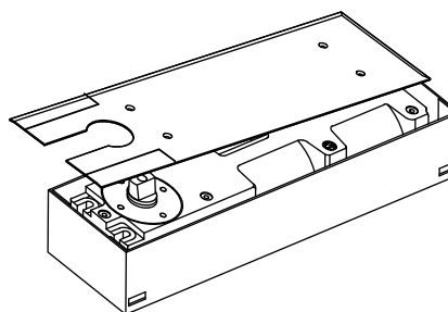
Standard Duty Floor Closer (FC-6280)
