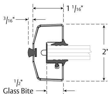
3/16" WEATHERING CLADDE
