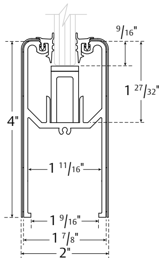
4", 6" Sidelite Rails = 9/16" Bite Top and Bottom
