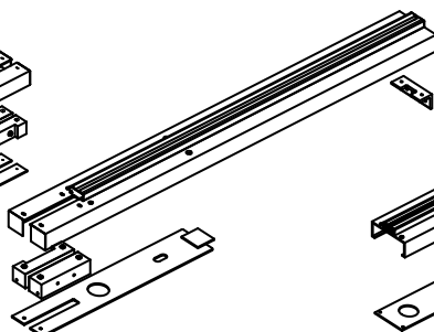
Floating Header (HDF-1750x4500-OHC) Sidelite Left
