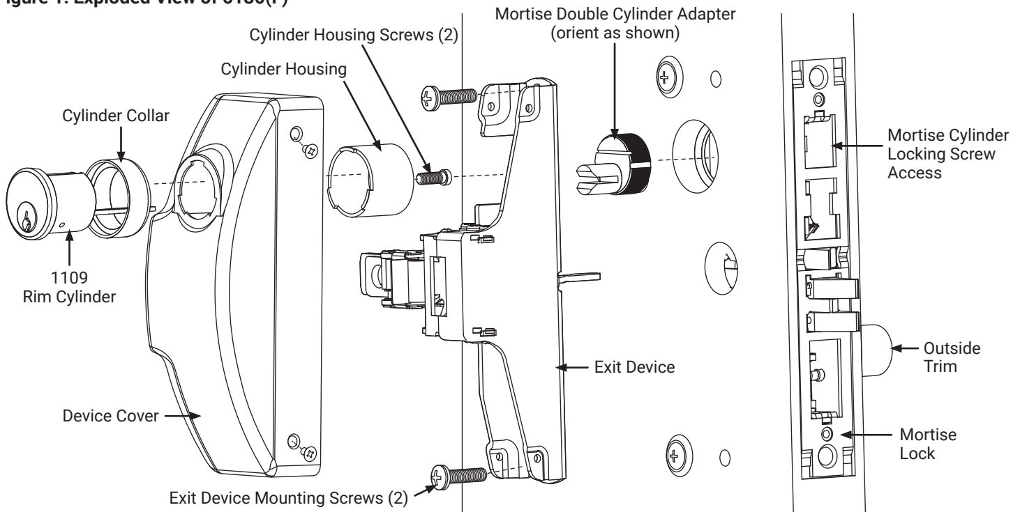
Figure 1: Exploded View of 6130(F)
