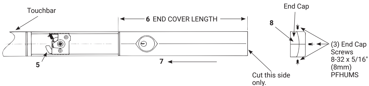
FIGURE B: DEVICE WITH CYLINDER DOGGING
