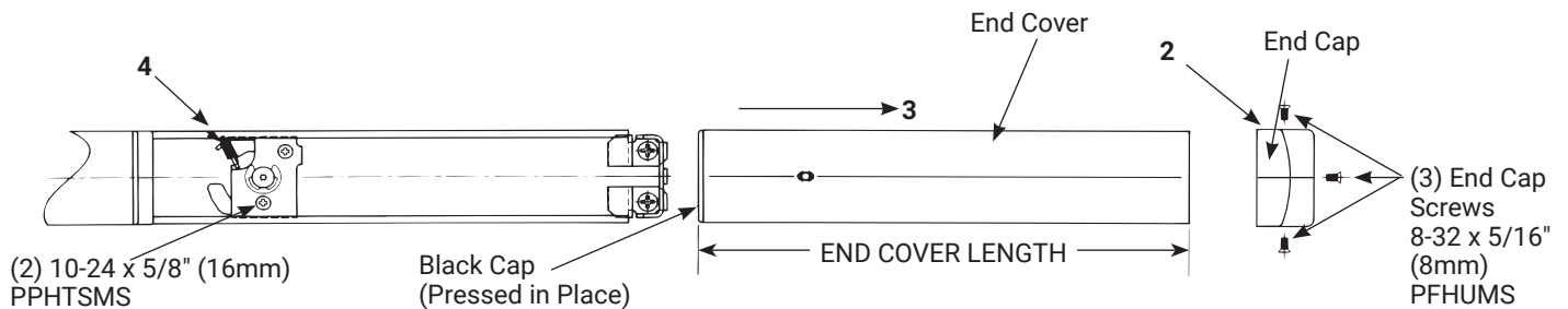
FIGURE A: DEVICE WITH STANDARD DOGGING
