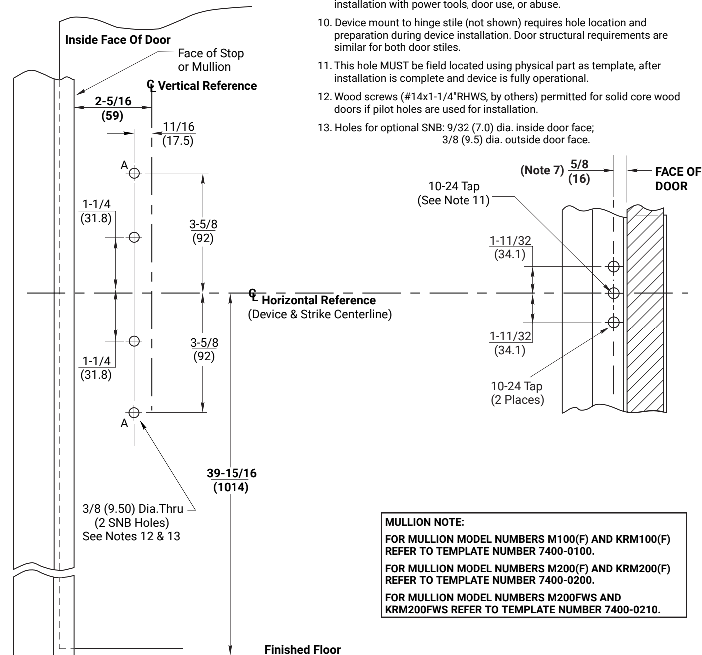
Strike Reinforcement (See Note 6)
