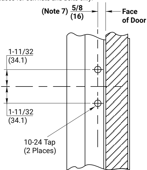
Strike Preparation Detail
