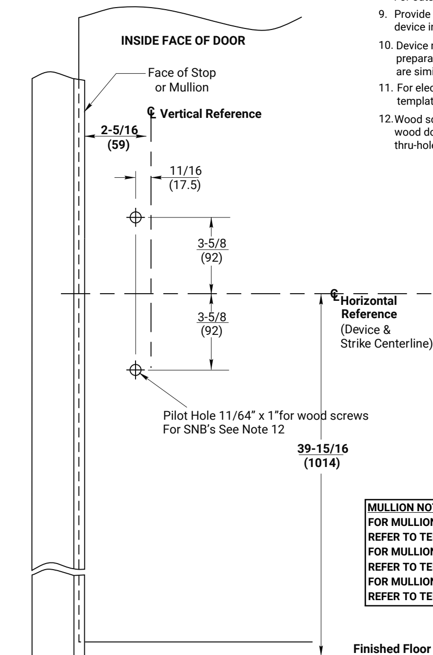
Strike Reinforcement (See Note 6)
