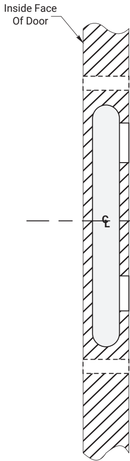
Section X - X
