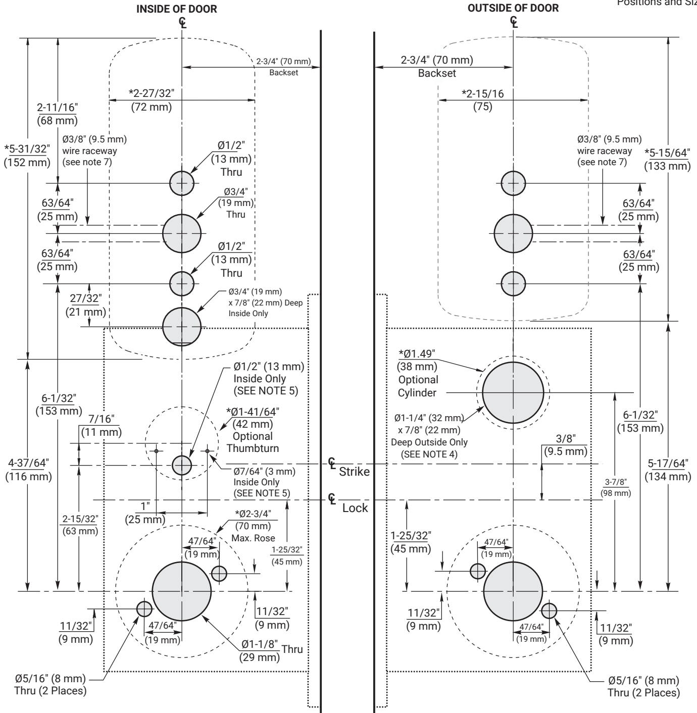
(*) Escutcheon & Trim Positions and Sizes
