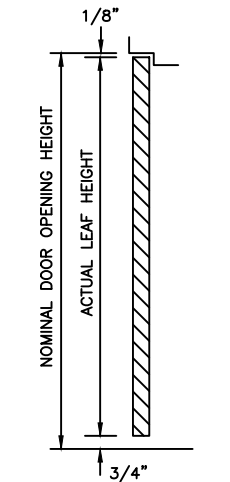
VERTICAL SECTION
