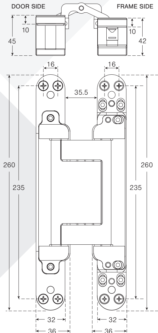
Hinge Dimensions (millimeters)
