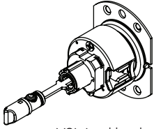
VSL Lockbody 1-3/8" - 2" Door
