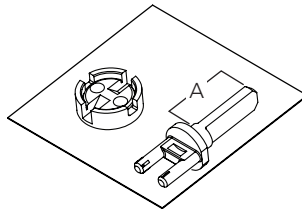
10-3635 (A=0.826") 10-3636 (A=0.989")
