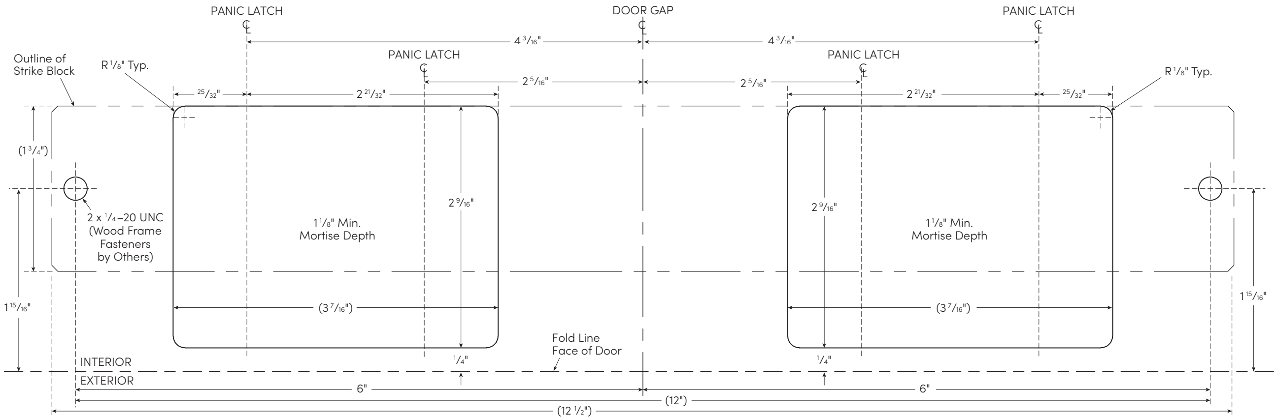
VIEW LOOKING UP Double Storefront, Wood, Metal Door.
