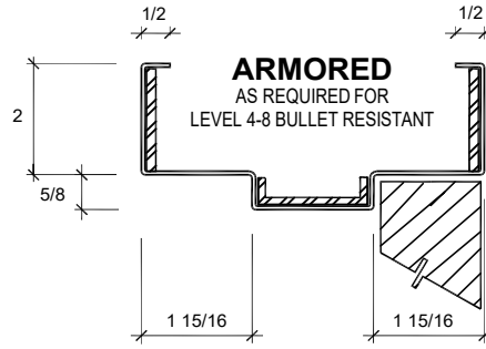
BULLET LEVEL 4-8 FRAME PROFILE
