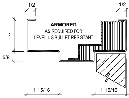
BULLET LEVEL 4-8 FRAME PROFILE
