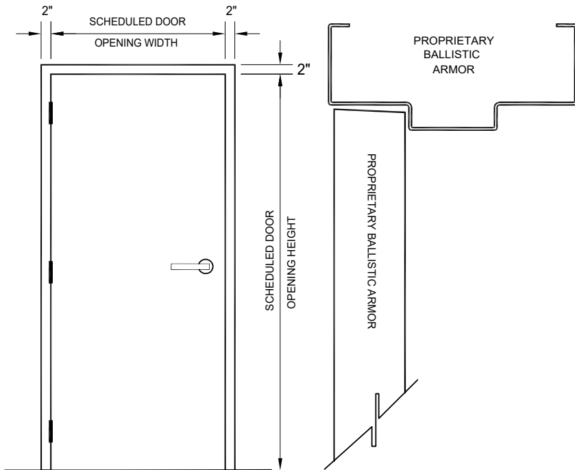
BULLET LEVEL 4-8 FRAME PROFILE
