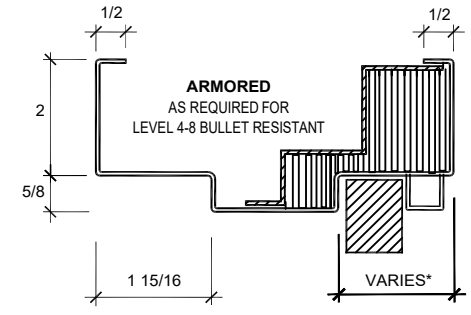
BULLET LEVEL 4-8 LITE PROFILE
