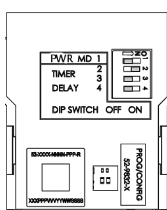
DIP Switch Setting for Timer Mode Installation
