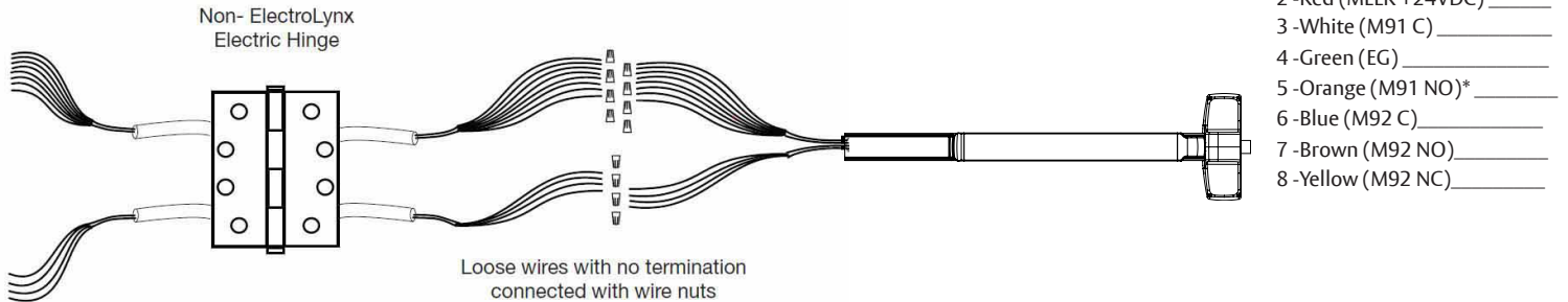
Figure 5 Non-ElectroLynx Power Mode Wiring
