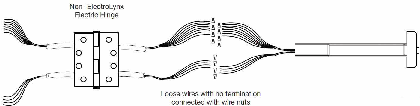
Figure 10 Timer Mode Installation
