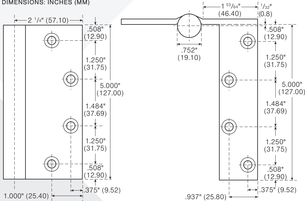
Center & Bottom Hinge Detail
