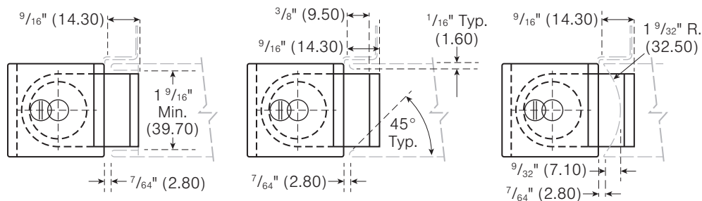
Suggested Hollow Metal Door Preparation
