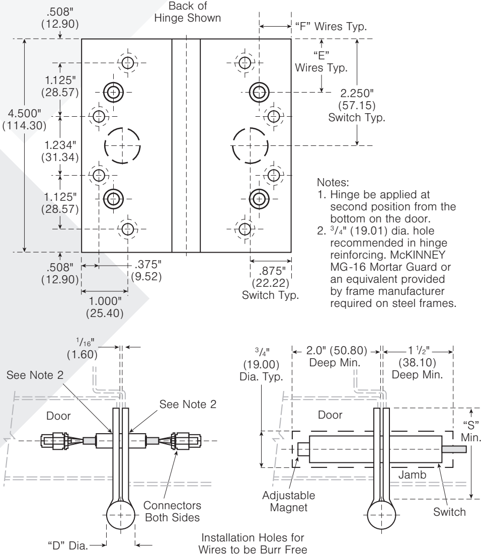
Top View Section through Wires (Hinge in Closed Position)
