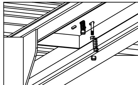
Figure 9.2: Spring Installation
