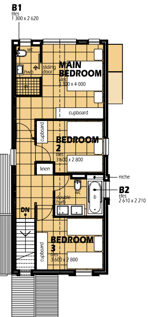
FIRST FLOOR LAYOUT
