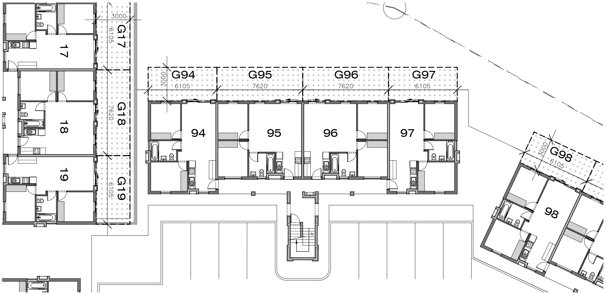
Ground Storey Exclusive Use Garden Areas: BUILDING 13 (BLOCK I) 1:200
