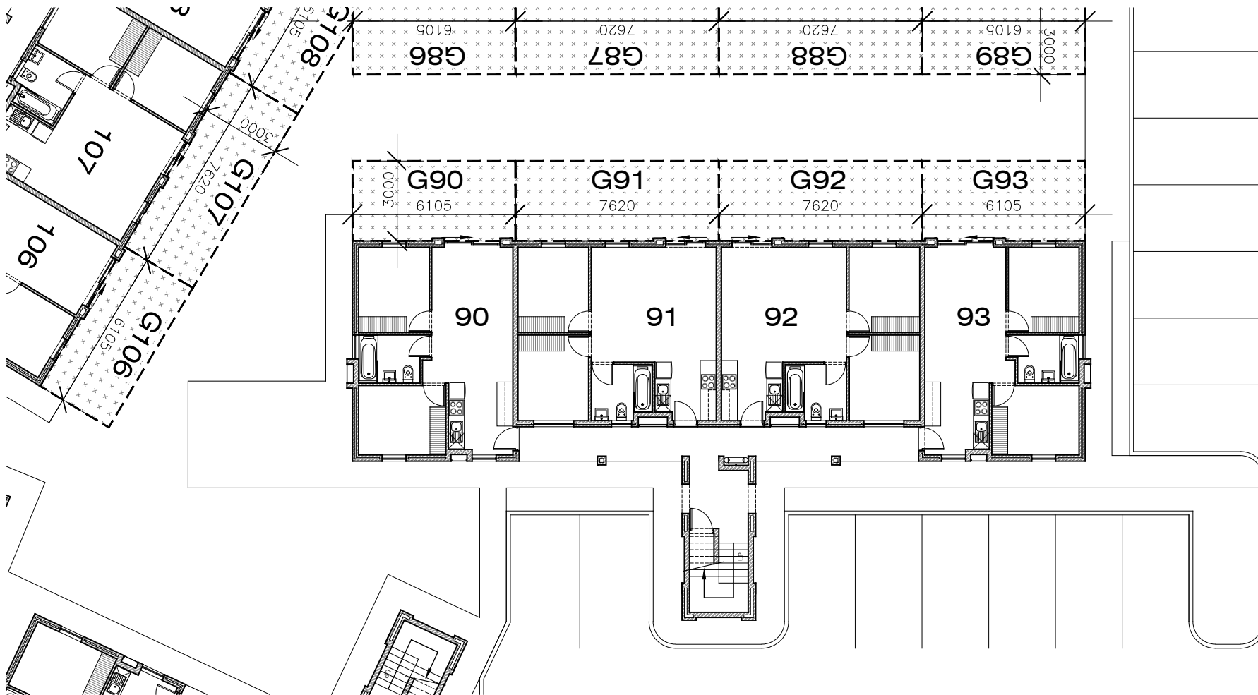
Ground Storey Exclusive Use Garden Areas: BUILDING 12 (BLOCK K) 1:200
