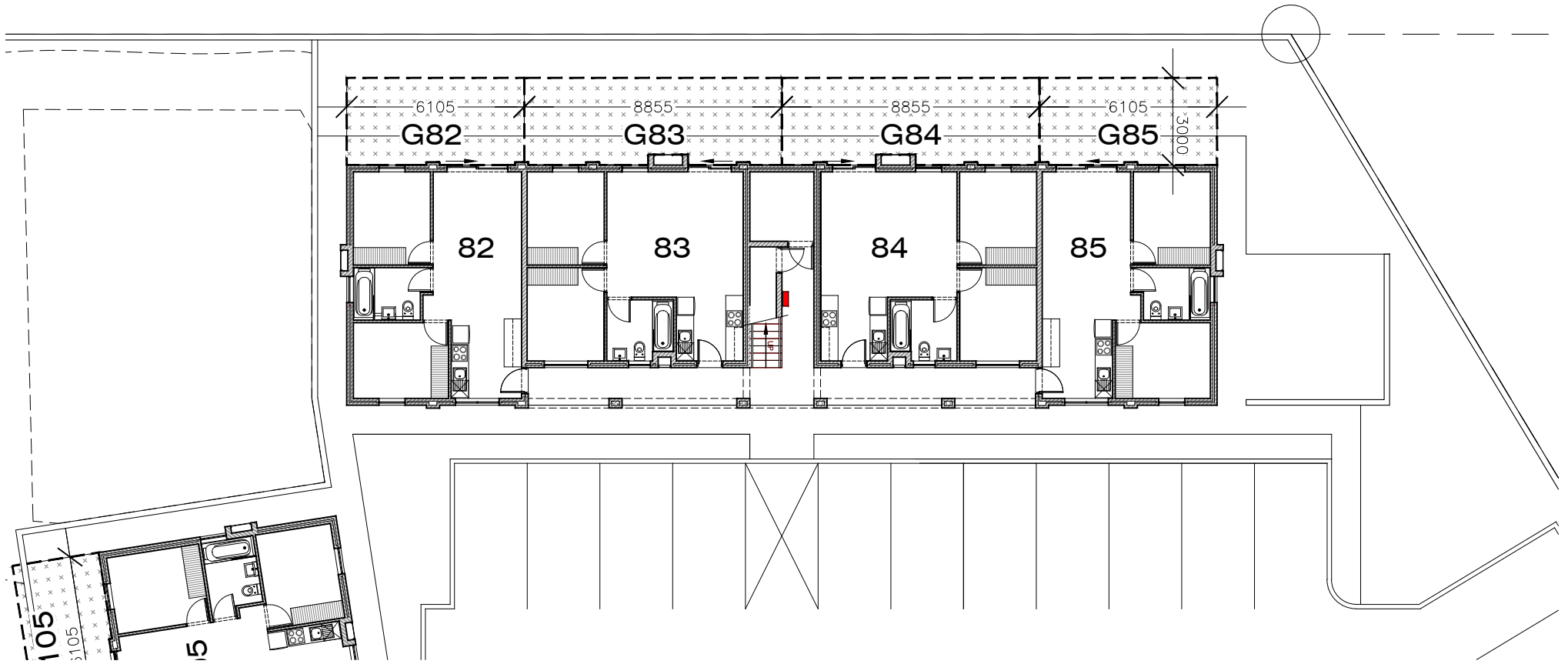
Ground Storey Exclusive Use Garden Areas: BUILDING 10 (BLOCK O) 1:200
