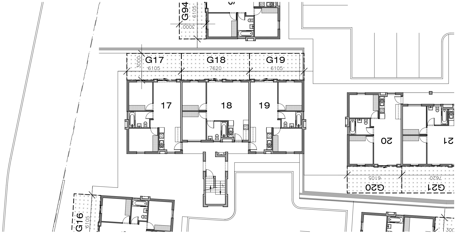
Ground Storey Exclusive Use Garden Areas: BUILDING 7 (BLOCK D) 1:200
