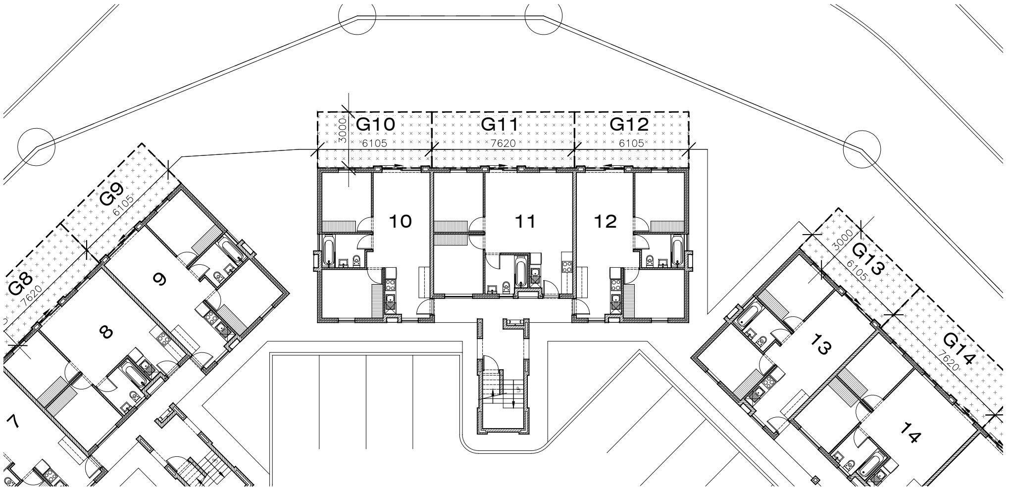
Ground Storey Exclusive Use Garden Areas: BUILDING 5 (BLOCK B) 1:200
