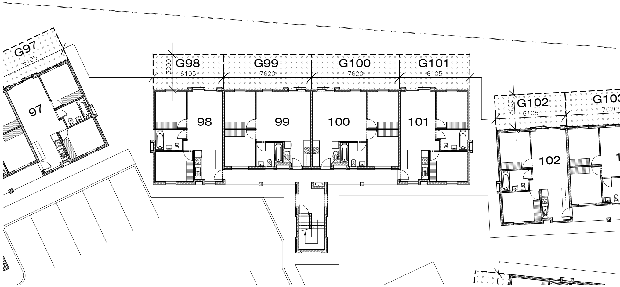
Ground Storey Exclusive Use Garden Areas: BUILDING 14 (BLOCK J) 1:200
