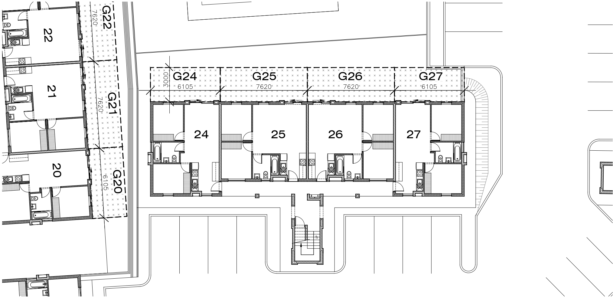
Ground Storey Exclusive Use Garden Areas: BUILDING g (BLOCK E) 1:200
