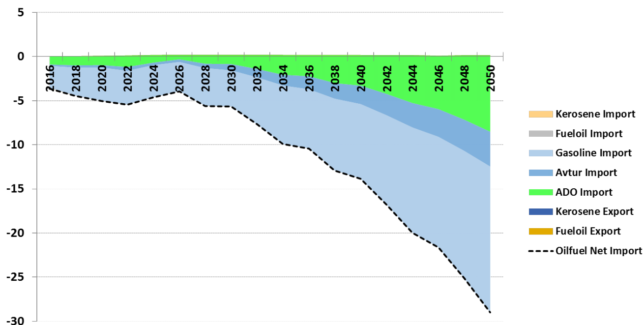
Figure 3.5 Export and import of oil fuels
