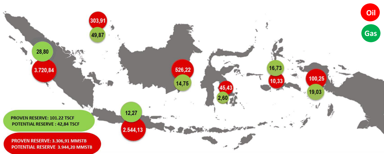
Figure 3.1 Oil and gas resources
