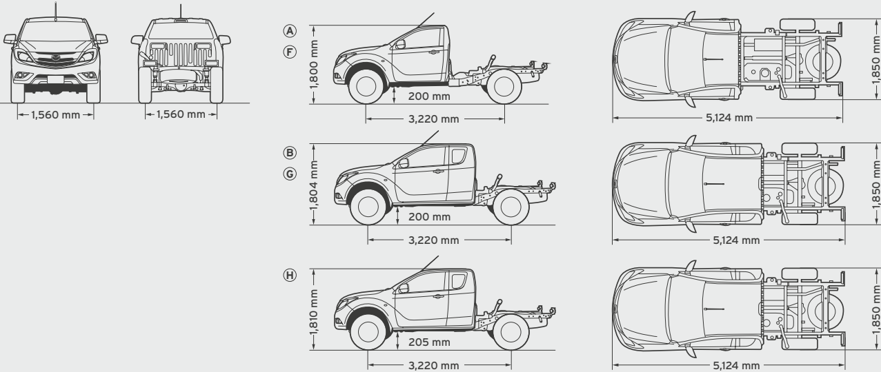
Chassis
