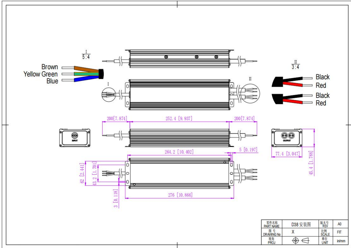
12V Version
