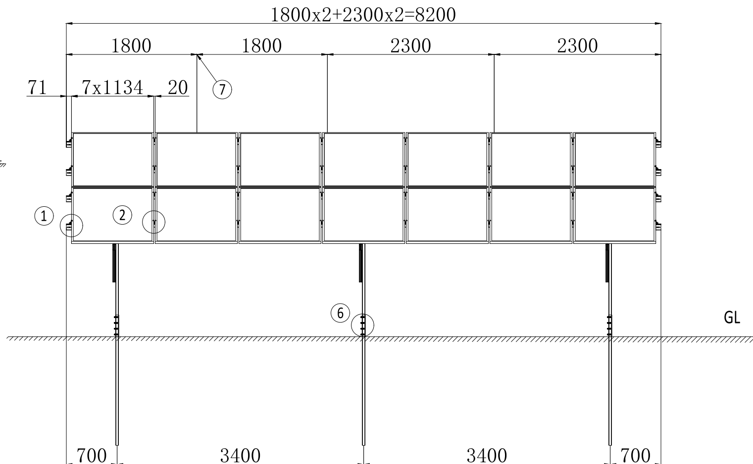
2*7*1 Array Front View
