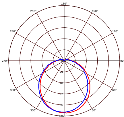
Photometric Diagram
