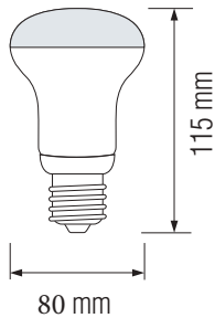
Technical Drawing
