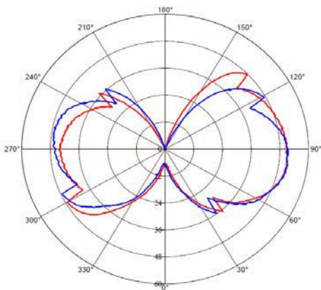
Photometric Diagram
