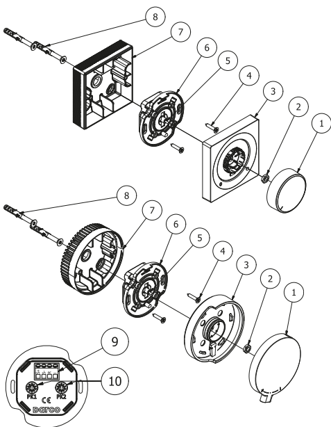
Figure 1. Regulators construction
