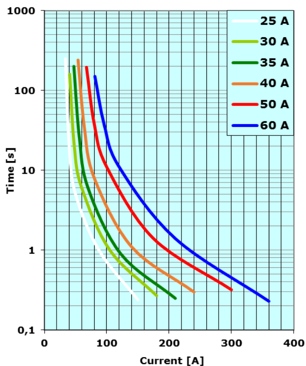
MaxiCompact® Operating Time @ 23°C test module ISO
