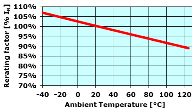
MaxiCompact® Derating Curve on test module ISO
