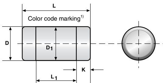
DIMENSIONS - MELF resistor types, mass and relevant physical dimensions
