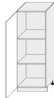
D5D 60 / 154 (600/1540/565)
