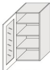
W4S 45 (450/960/325)
