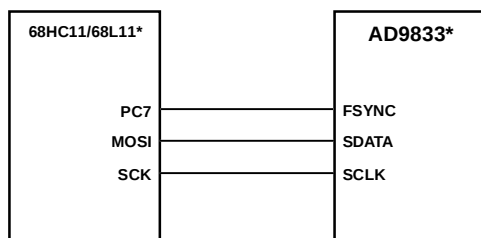
Figure 10. 68HC11/68L11 to AD9833 Interface
