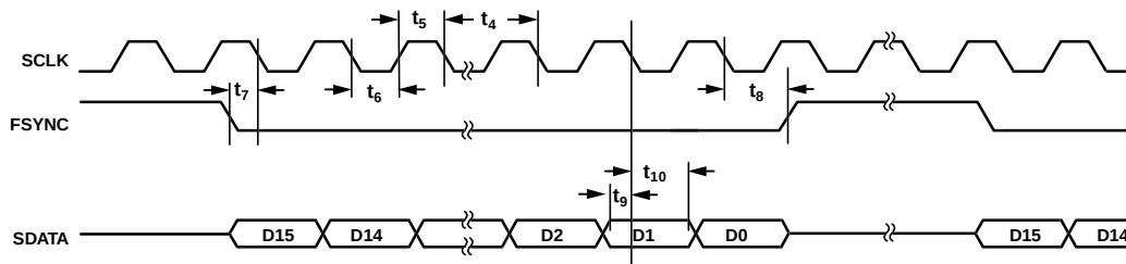
Figure 3. Serial Timing
