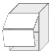
W8B 60 AVENTOS (600/720/325)
