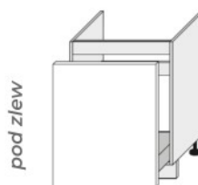
D1ZR 60 (600/820/500)
