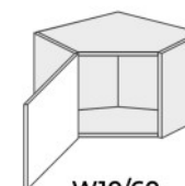
W10/60 (600/360/600)
